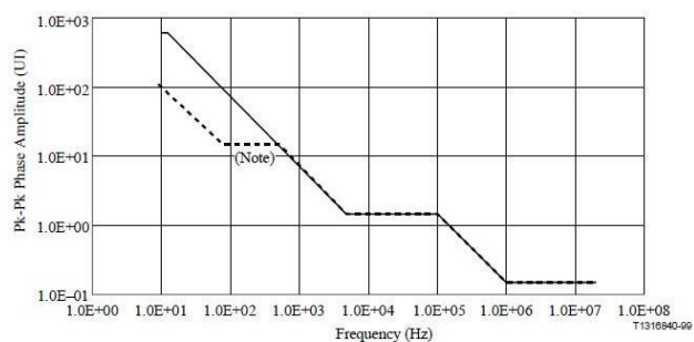
Figure 4/G.825 – STM-16 jitter tolerance
