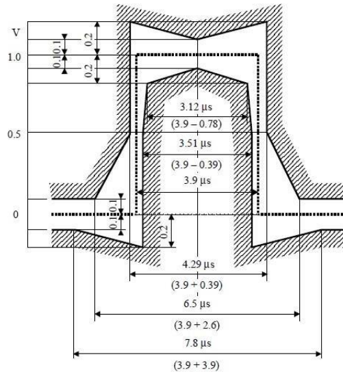
a) Mask for single pulse
