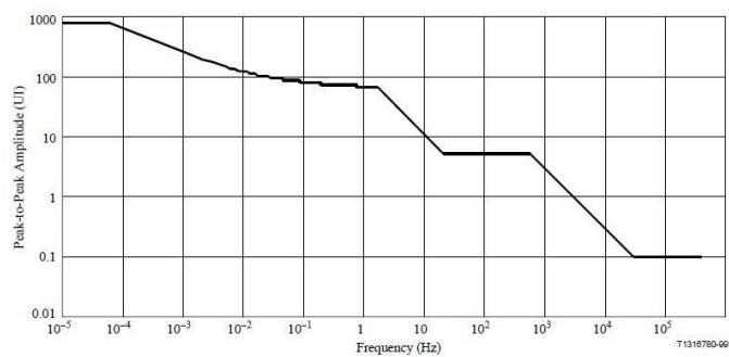
Figure 9/G.824 – Jitter and wander tolerance of 44 736 kbit/s input ports
