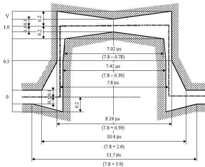
b) Mask for double pulse
