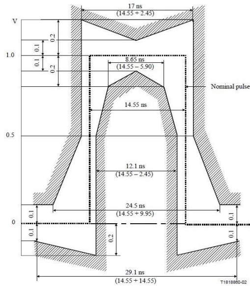
Figure 17/G.703 – Pulse mask at the 34 368 kbit/s interface
